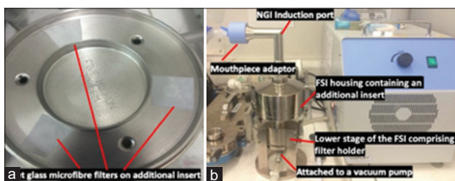
Figure 1: Fast Screening Impactor (a) three pieces of wet glass microfibre filters covered on additional insert and (b) the experimental setup
